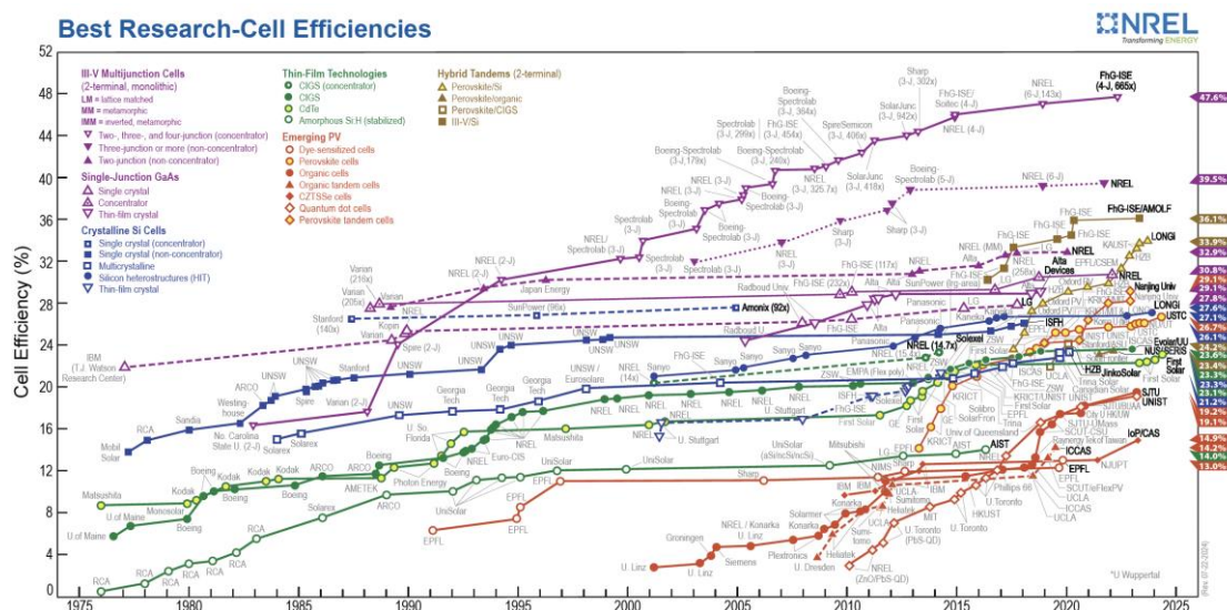
Figure 7-7: Evolution in solar cell efficiency 1975 - 2024 [Ref. 81]
